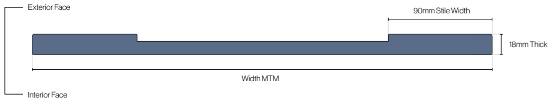
Hartford Door Cross Section
