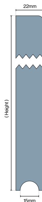
Hidden Profile Handle Slab Door Cross Section
