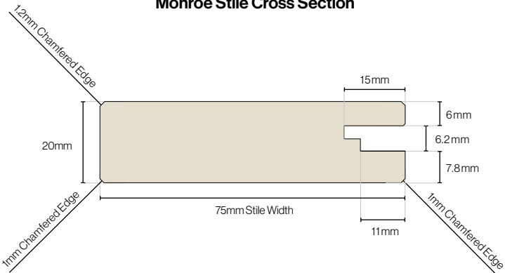
Monroe Stile Cross Section
