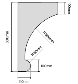
French Mantle Corbel 350mm (L) x 90mm (H) x 600mm (H)
