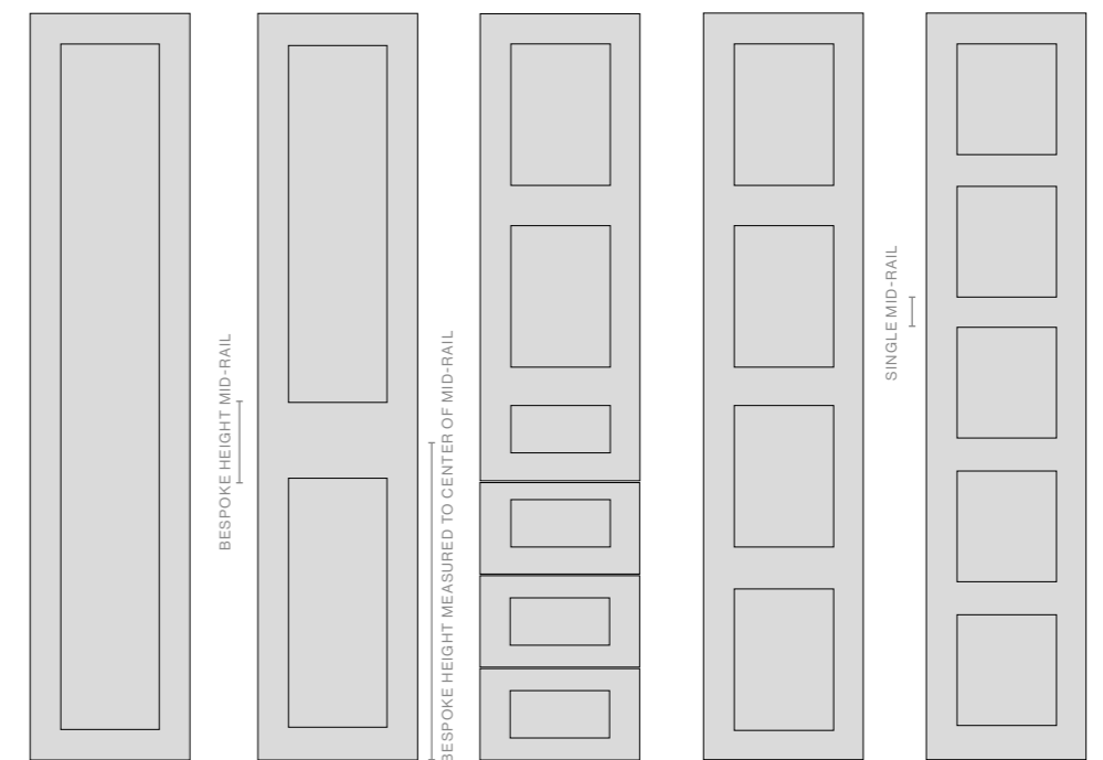
5G Bedroom Single Panel Door, 5G Bedroom Bespoke Height Mid-rail Door, 5G Bedroom 3 Panel Stable Door, 5G Bedroom 4 Panel Door, 5G Bedroom 5 Panel Door
