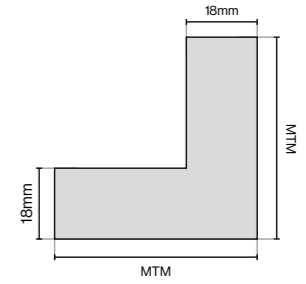
MTM Corner Post 715mm (150 x 150mm Max)
