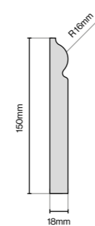
Torus Plinth 3050mm Lengths
