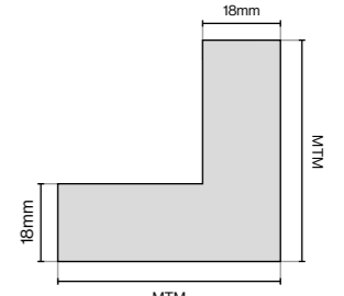
MTM Corner Post 715mm (150 x 150mm Max)
