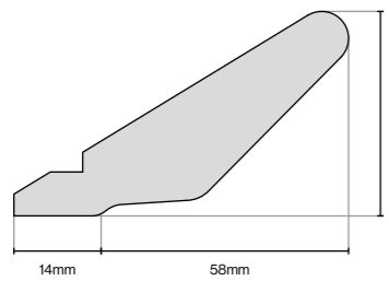
Tangent Cornice 3050mm Lengths
