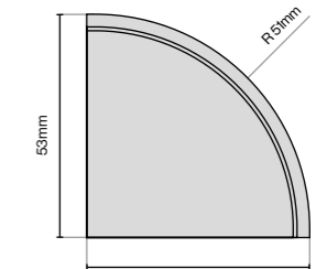
Under Cornice Quadrant (Smooth) 53mm (L) x 53mm (W) x 30mm (H)
