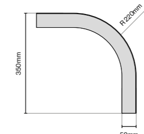
Curved Modern Cornice / Pelmet 350mm (L) x 350mm (W) x 30mm (H)
