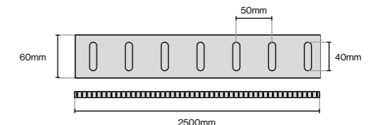
Fluted Rail 2500mm (L) x 18mm (W) x 60mm (H)
