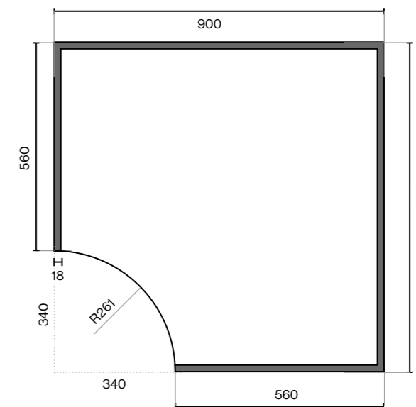
340mm Concave Door 340mm x 340mm Concave Door for 900mm Base Unit
